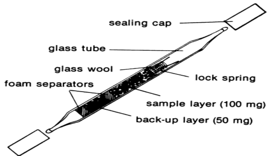
Fig. (4): Standard activated charcoal tube used inorganic vapor sampling
